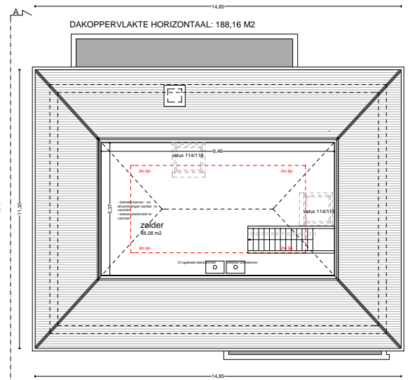
ZOLDER
