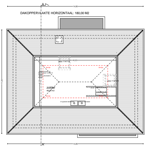
ZOLDER
