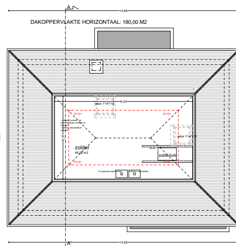
ZOLDER
